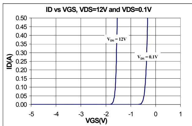
Figure 6 – Transfer Characteristic
