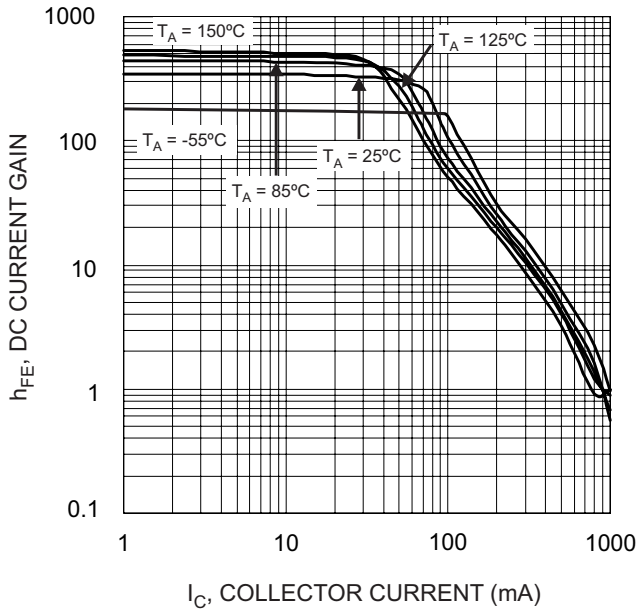
Fig. 5, Typical DC Current Gain vs. Collector Current
