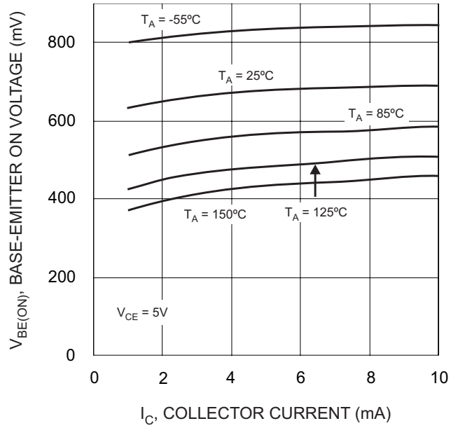
Fig. 4, Typical Base-Emitter Turn-On Voltage vs. Collector Current
