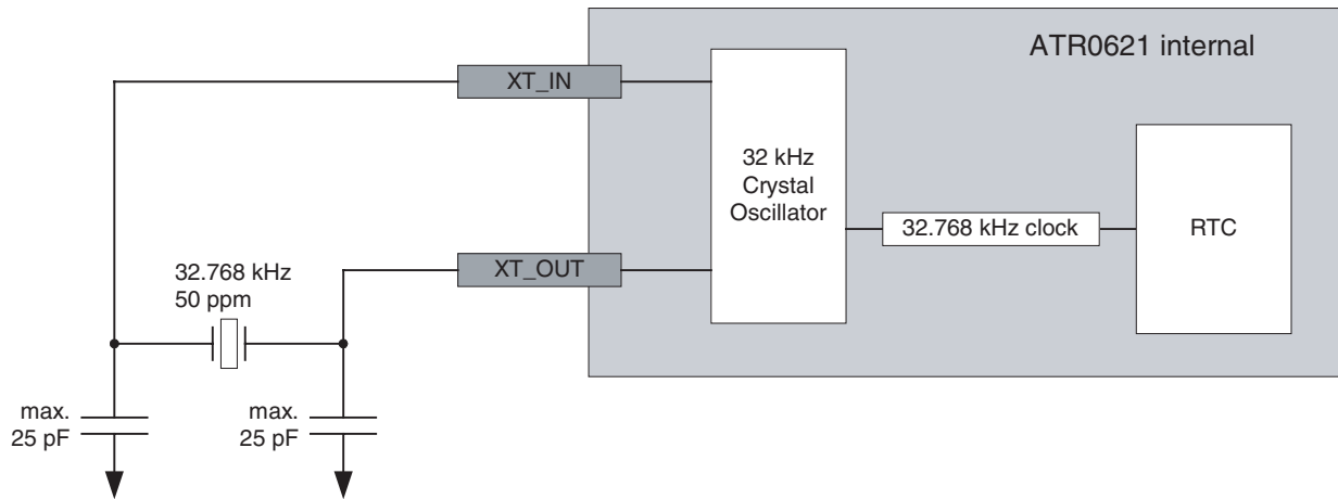
Figure 4-1. Crystal Connection
