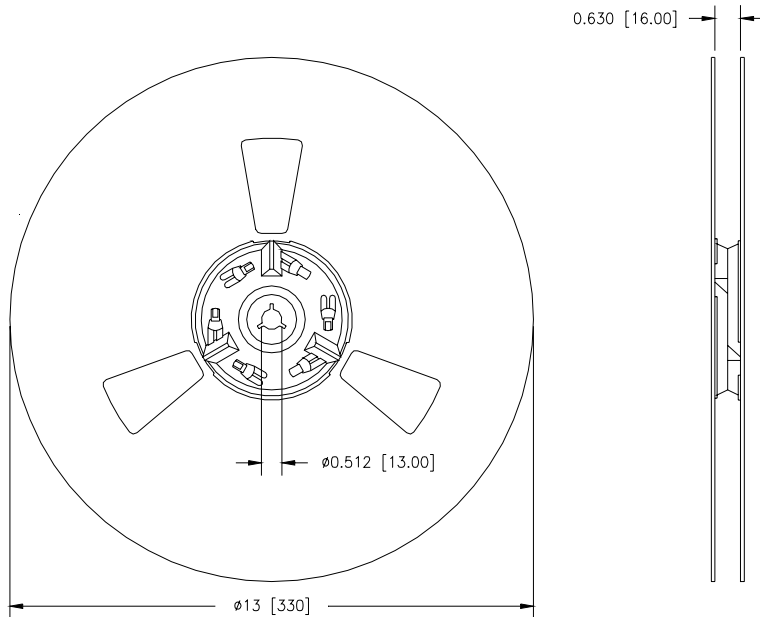
Figure 21: Reel Dimensions
