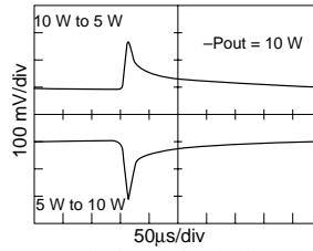
MHD2815D +Vout Step Load Response
