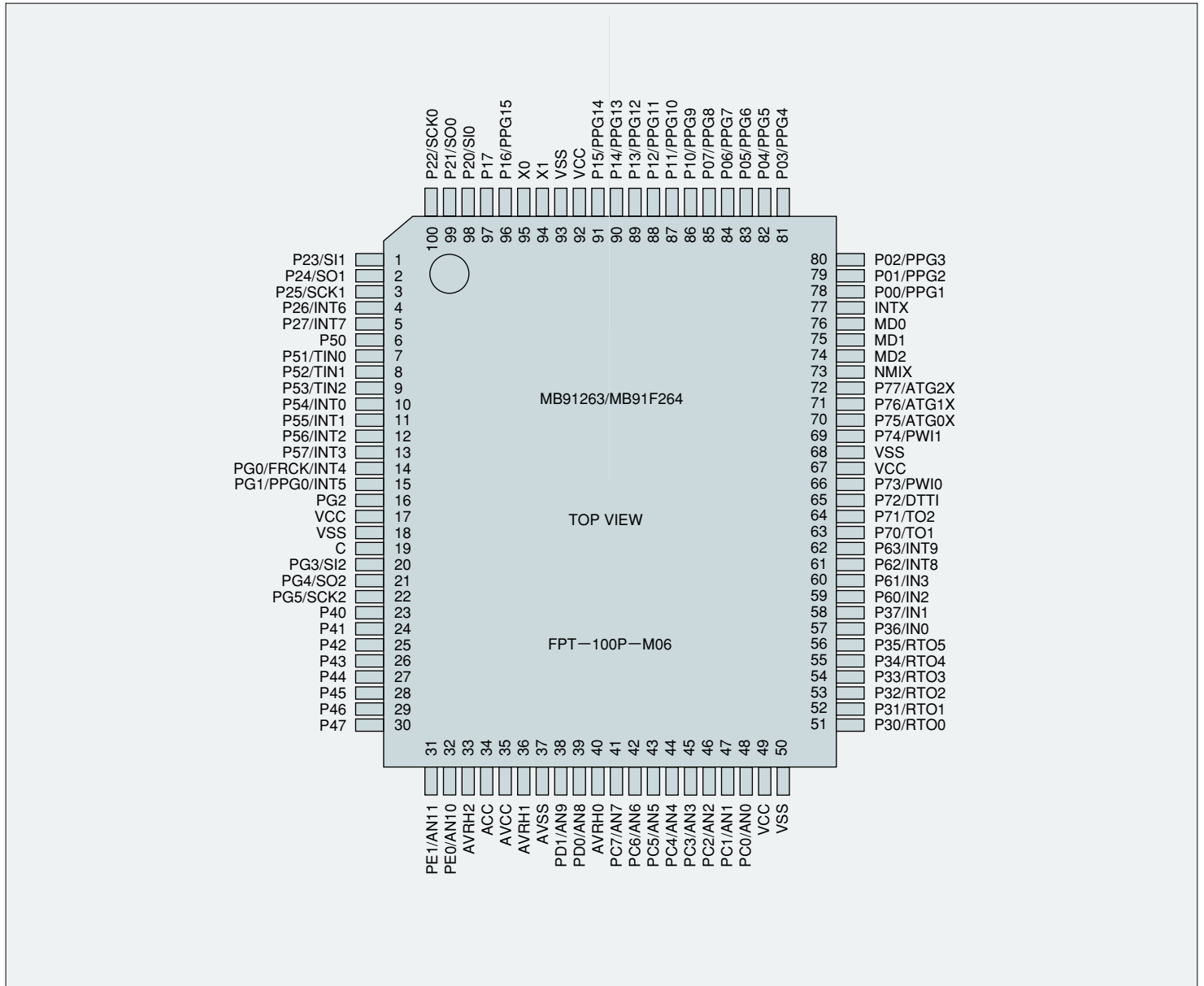
Figure 5 Pin Assignments
