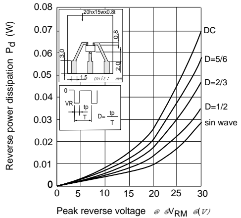
Fig.4. Reverse power dissipation Vs. Peak reverse voltage
