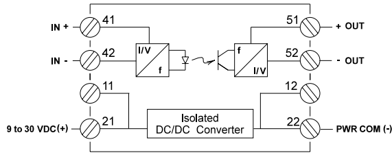
Figure 1: G408 Block Diagram
