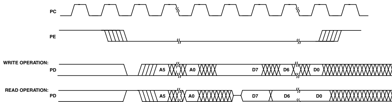
Figure 1. SPI Timing
