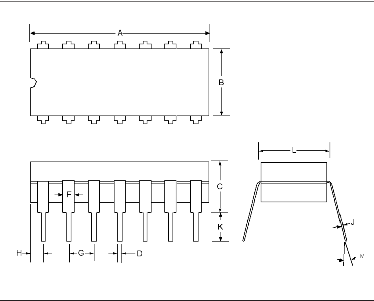
J 14-Pin Ceramic Dip
