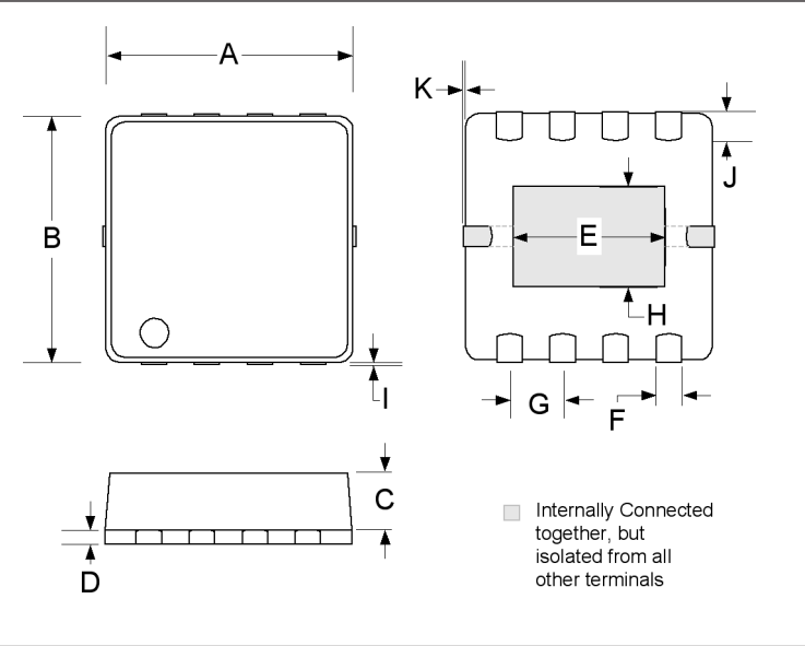
LM 8-Pin Plastic MLP-Micro Exposed Pad
