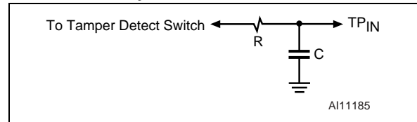
Figure 21. Low Pass Filter Implementation for Noise Immunity
