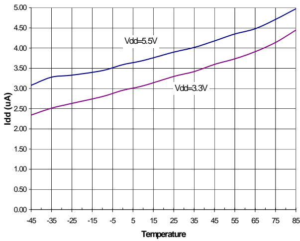
FIGURE 7. I_{DD3} vs TEMPERATURE
