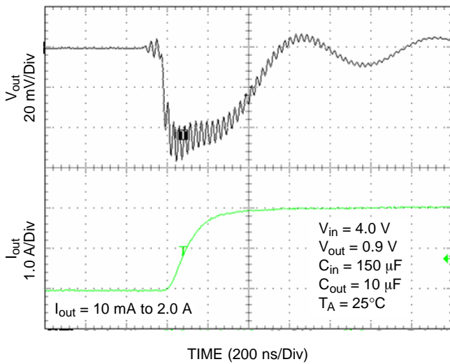
Figure 15. Load Transient Response
