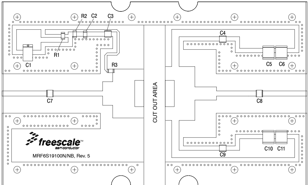
Figure 2. MRF6S19100NR1(NBR1) Test Circuit Component Layout
