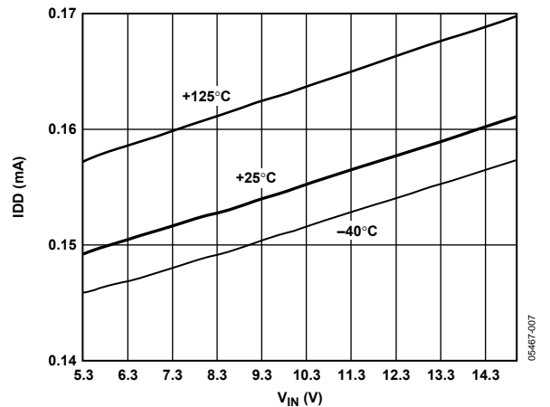
Figure 7. ADR365 Supply Current vs. Input Voltage
