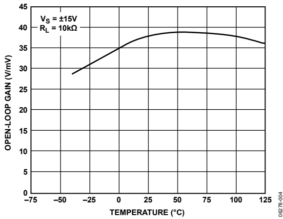
Figure 4. AD8682 Open-Loop Gain vs. Temperature
