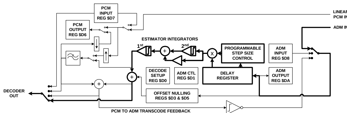
Figure 4 ADM Decoding
