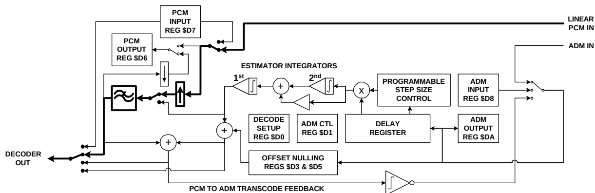
Figure 6 PCM Decoding
