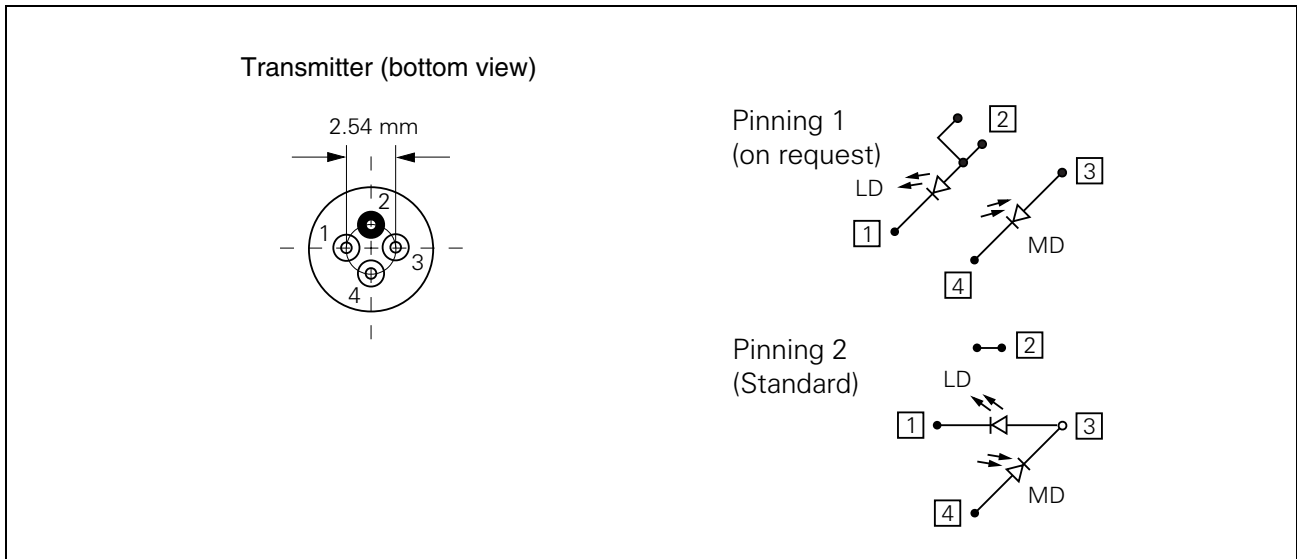
Figure 1 Transmitter
