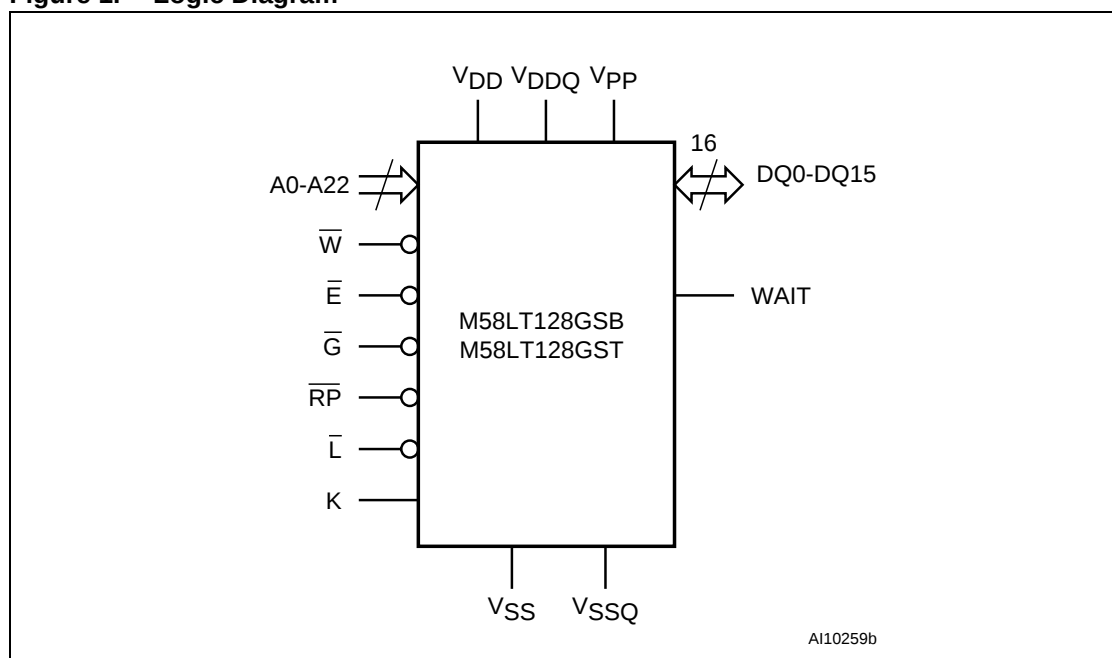
Figure 1. Logic Diagram
