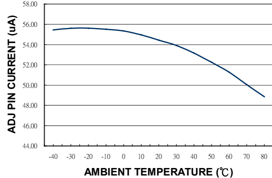
ADJ PIN CURRENT vs. AMBIENT TEMPERATURE
