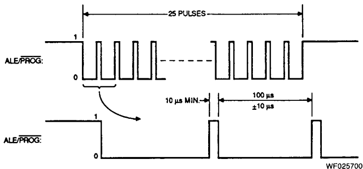
Figure 2. \overline{\text{PROG}} Waveforms
