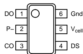
SOT23-6 (Top View)
