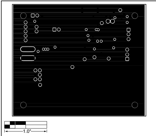
Figure 5. MAX3296 SW EV Kit PC Board Layout—Ground Plane
