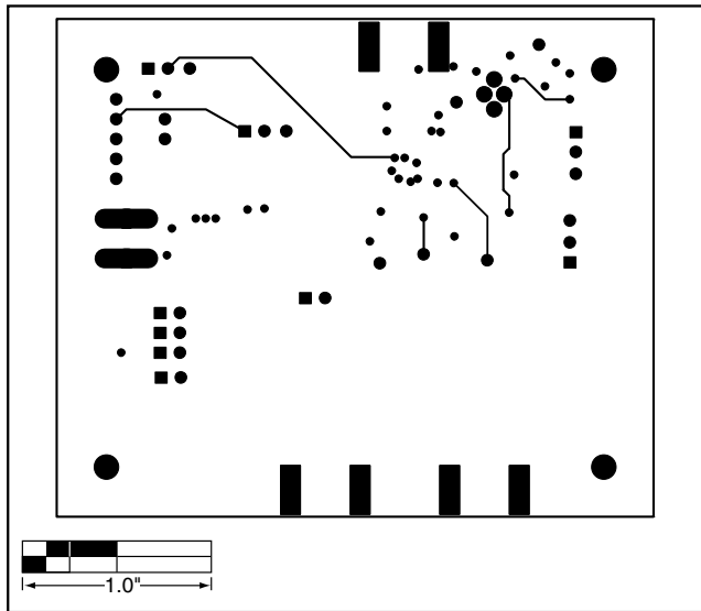
Figure 7. MAX3296 SW EV Kit PC Board Layout—Solder Side
