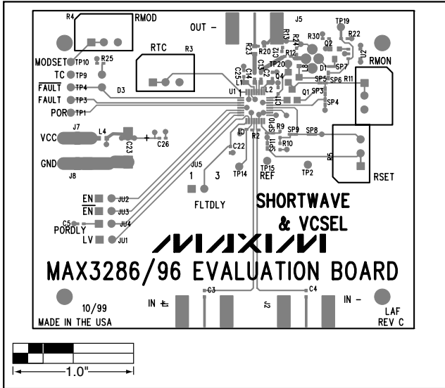
Figure 3. MAX3296 SW EV Kit Component Placement Guide—Top Silkscreen
