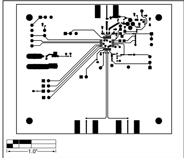
Figure 4. MAX3296 SW EV Kit PC Board Layout—Component Side
