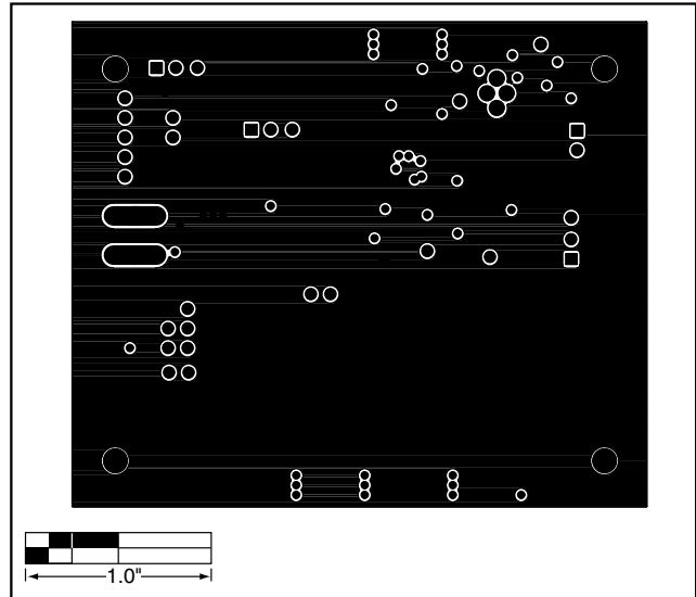
Figure 6. MAX3296 SW EV Kit PC Board Layout—Power Plane
