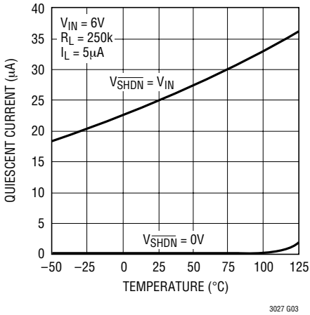
Quiescent Current
