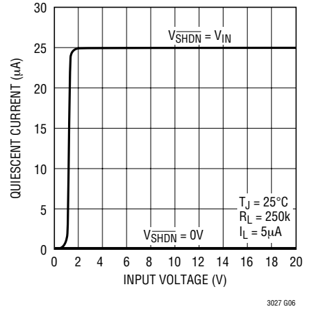
Quiescent Current
