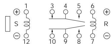
Double coil latch type (reset position)
