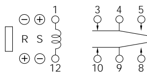
Single coil latch type (reset position)
