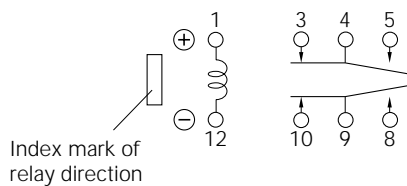
Non-latch type (not energized position)
