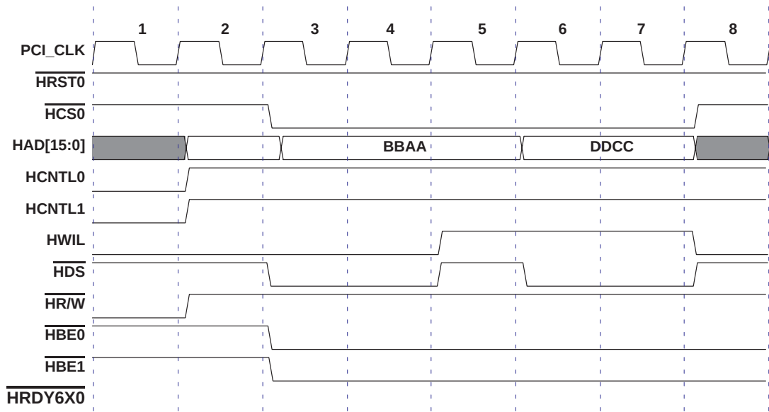
Figure 6–7. Double Word Read From HPID Without Auto-Increment Selected
