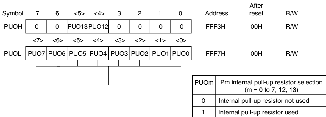
Figure 6-20. Format of Pull-up Resistor Option Register
