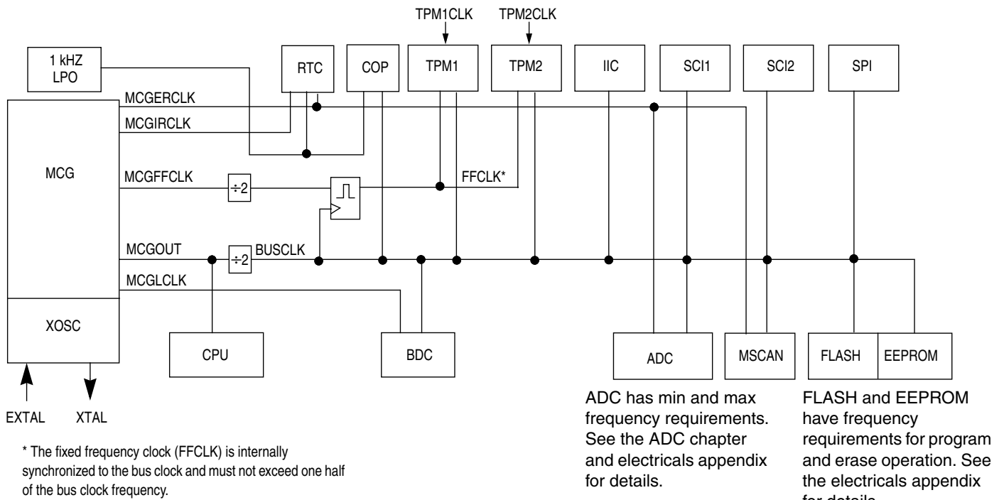
Figure 1-2. MC9S08DZ60 System Clock Distribution Diagram
