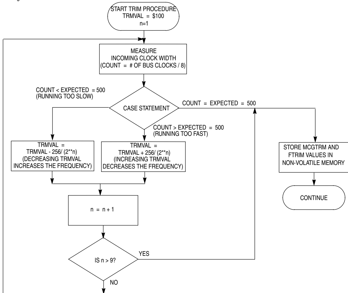
Figure 8-12. Trim Procedure
