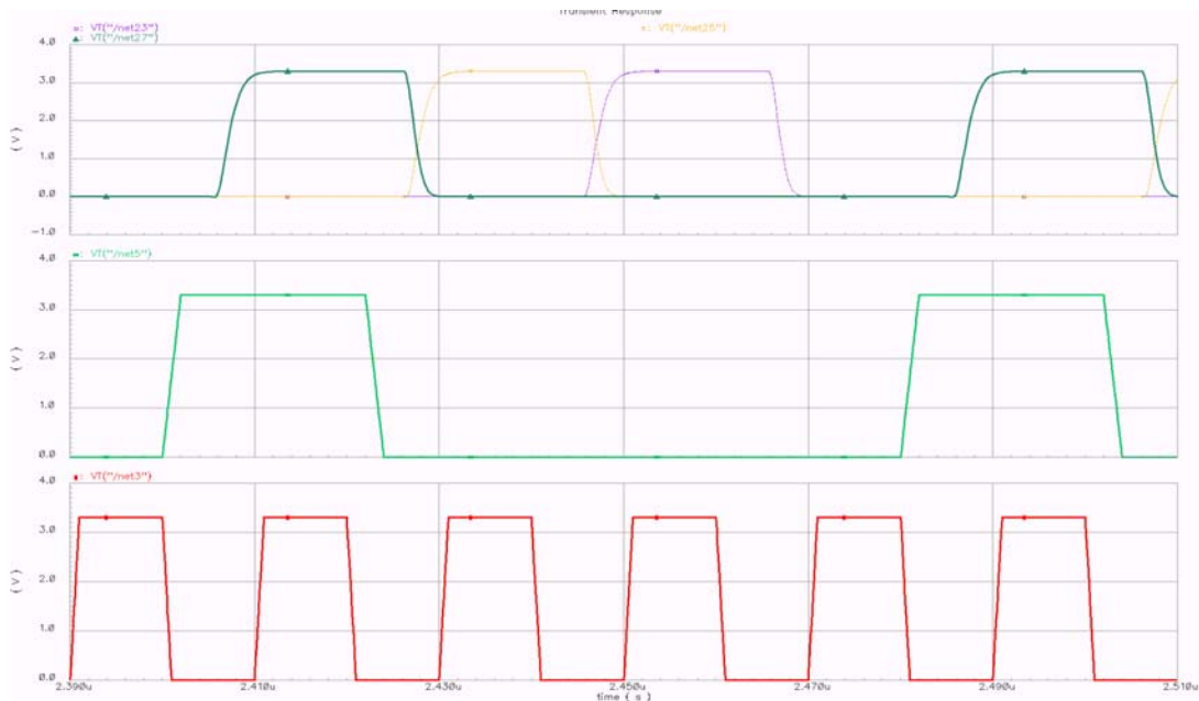
Figure 16: X-addressing. From bottom to top: Clock_x, Sync_x, internal selection pixel 1&2, internal selection pixel 3&4, internal selection pixel 5 & 6.
