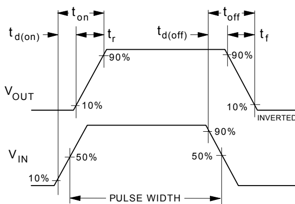
Figure 12. Switching Waveforms.
