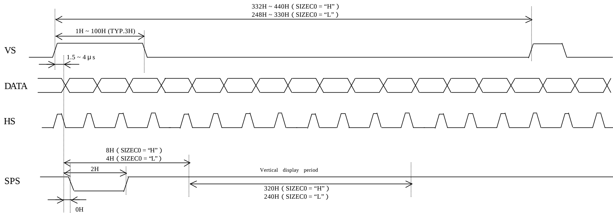
Fig.3 Vertical counter timing chart
