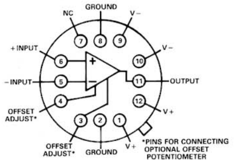
TO-8 PACKAGE BOTTOM VIEW
