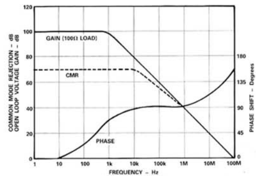
Figure 1. HOS-060 Frequency Response
