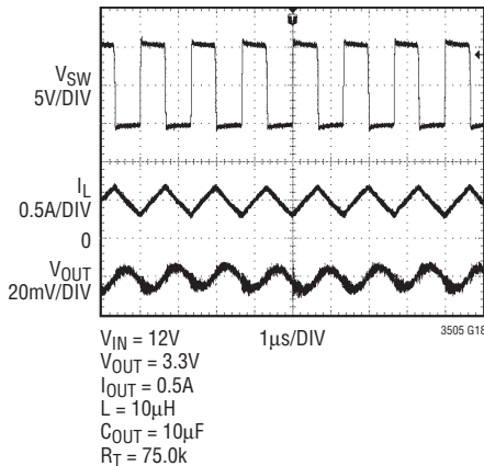
Operating Waveforms
