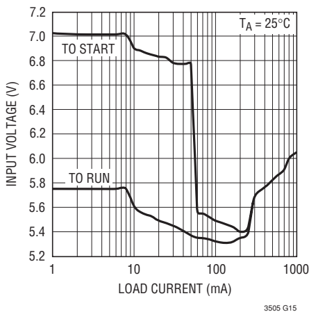
(7a) Typical Minimum Input Voltage, V_{OUT} = 5\text{V} , f_{SW} = 750\text{kHz}
