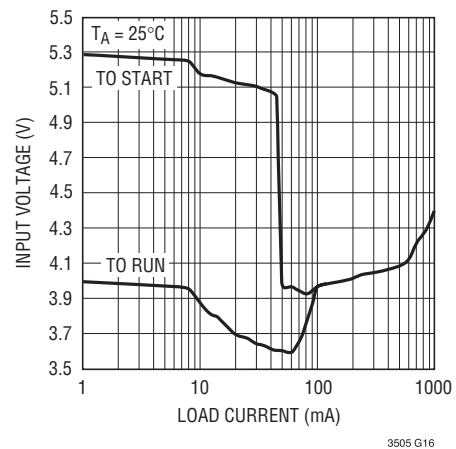
(7b) Typical Minimum Input Voltage, V_{OUT} = 3.3\text{V} , f_{SW} = 750\text{kHz}
