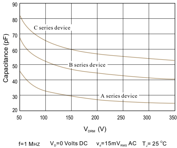
TYPICAL CAPACITANCE V.S. RATED REPETITIVE OFF-STATE VOLTAGE
