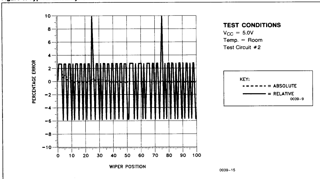
Figure 3: Typical Linearity for X9102
