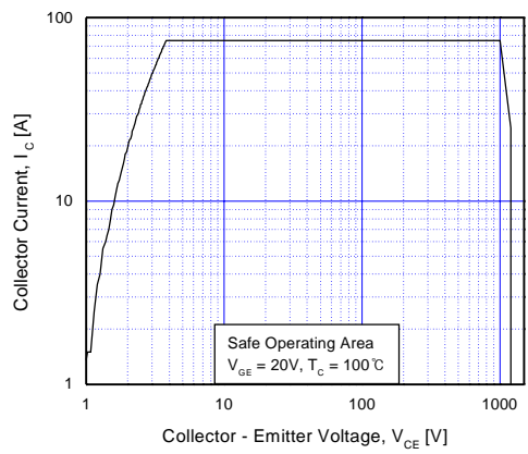
Fig 16. Turn-Off SOA
