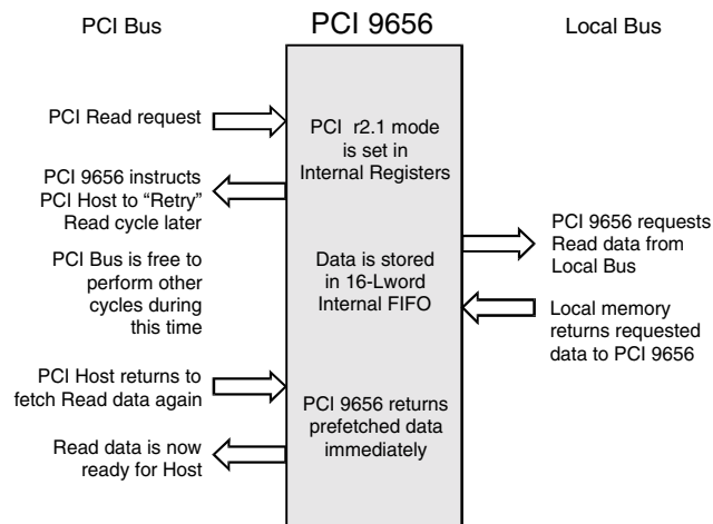
Figure 5-7. Direct Slave Delayed Reads
