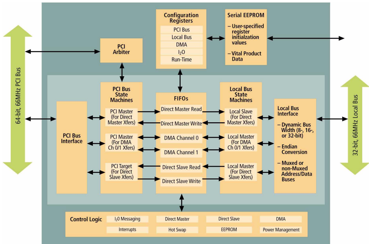
PCI 9656 Block Diagram
