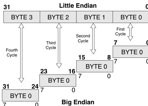
Figure 4-4. Big/Little Endian—8-Bit Local Bus
