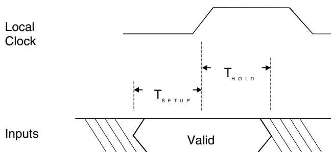
Figure 13-1. PCI 9656 Local Input Setup and Hold Waveform
