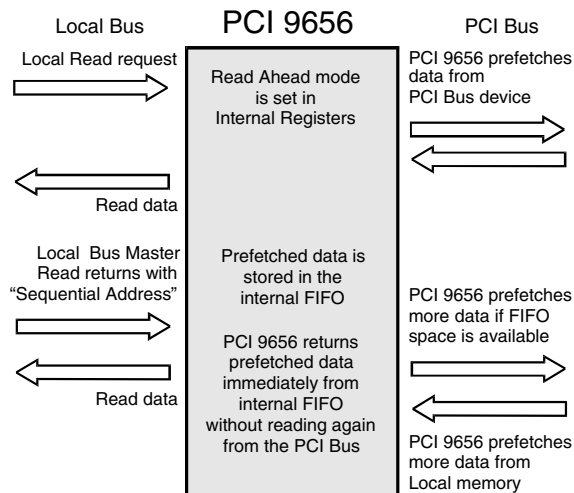
Figure 3-4. Direct Master Read Ahead Mode
