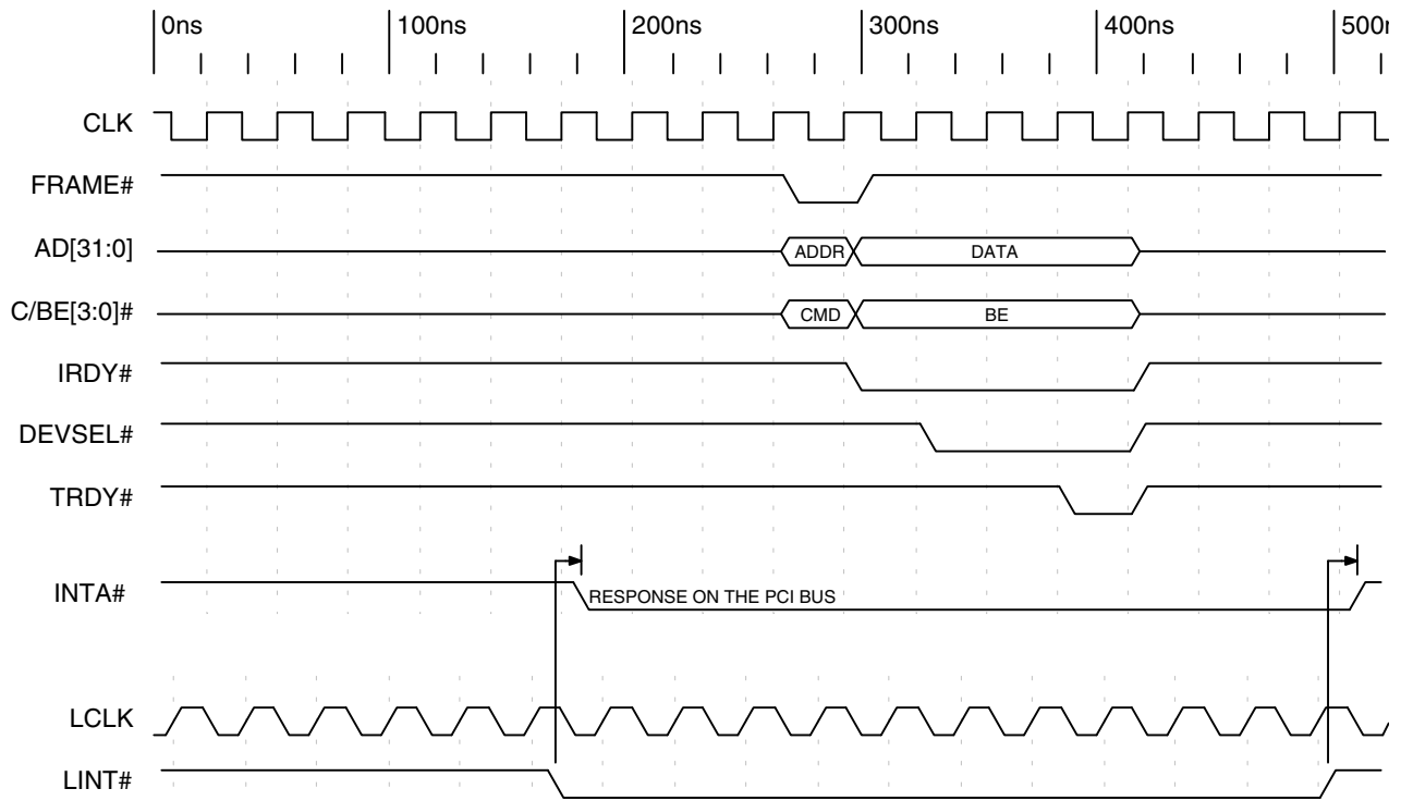
Timing Diagram 5-5. Local Interrupt Asserting PCI Interrupt
