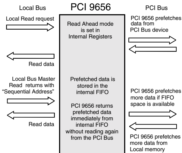
Figure 5-4. Direct Master Read Ahead Mode
