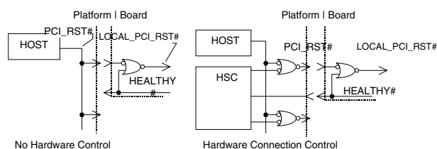
Figure 9-3. PCI Reset
