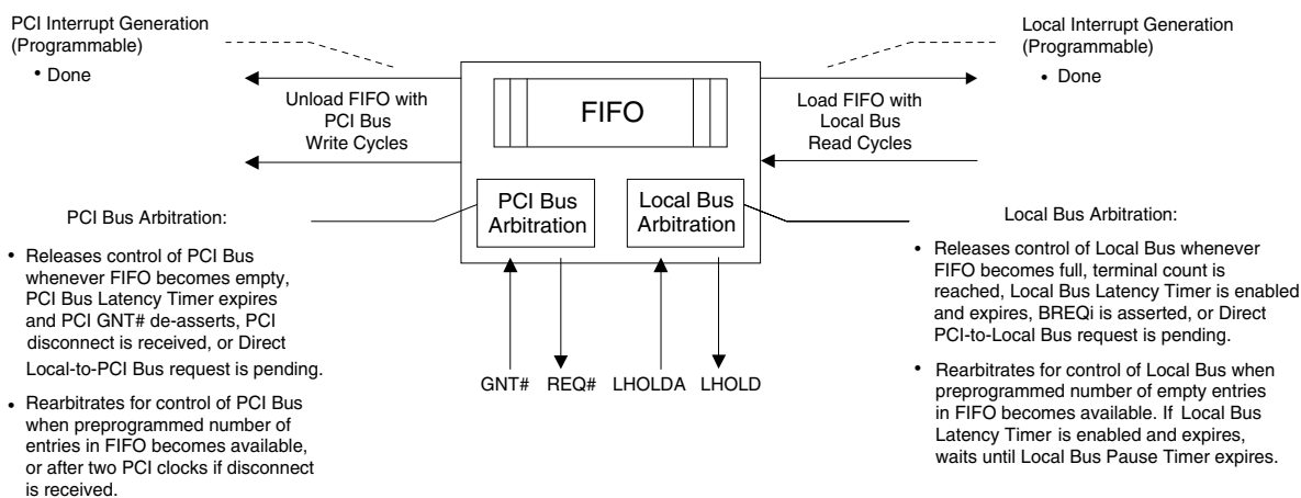
Figure 5-19. Local-to-PCI Bus DMA Data Transfer Operation
