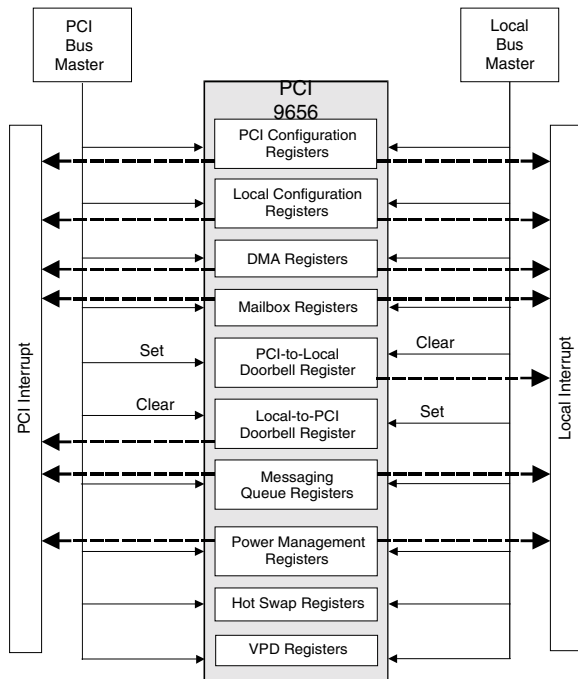
Figure 4-6. PCI 9656 Internal Register Access
