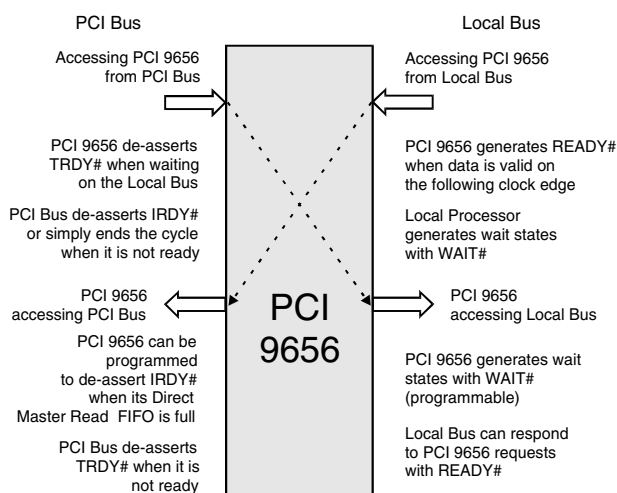
Figure 4-1. Wait States
