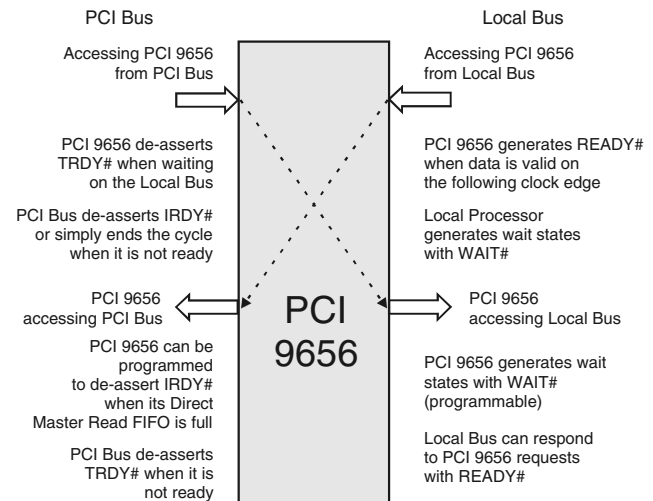
Figure 2-1. Wait States
