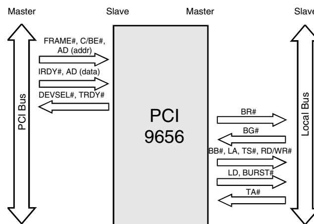
Figure 3-9. Direct Slave Write
