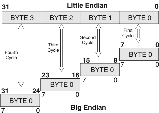
Figure 2-4. Big/Little Endian—8-Bit Local Bus
