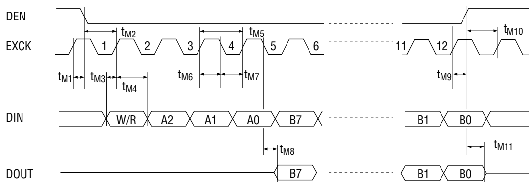
Figure 7 MCU Interface
