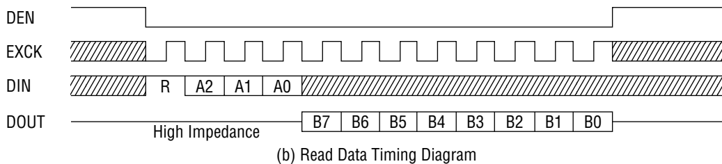
Figure 5 MCU Interface Input/Output Timing
