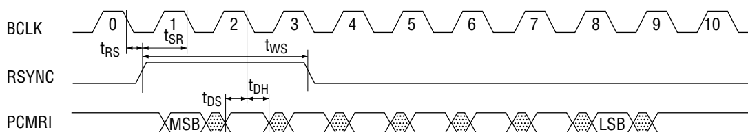
Figure 6 PCM Data Interface
