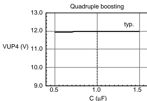
Figure 45 Booster (cont)
