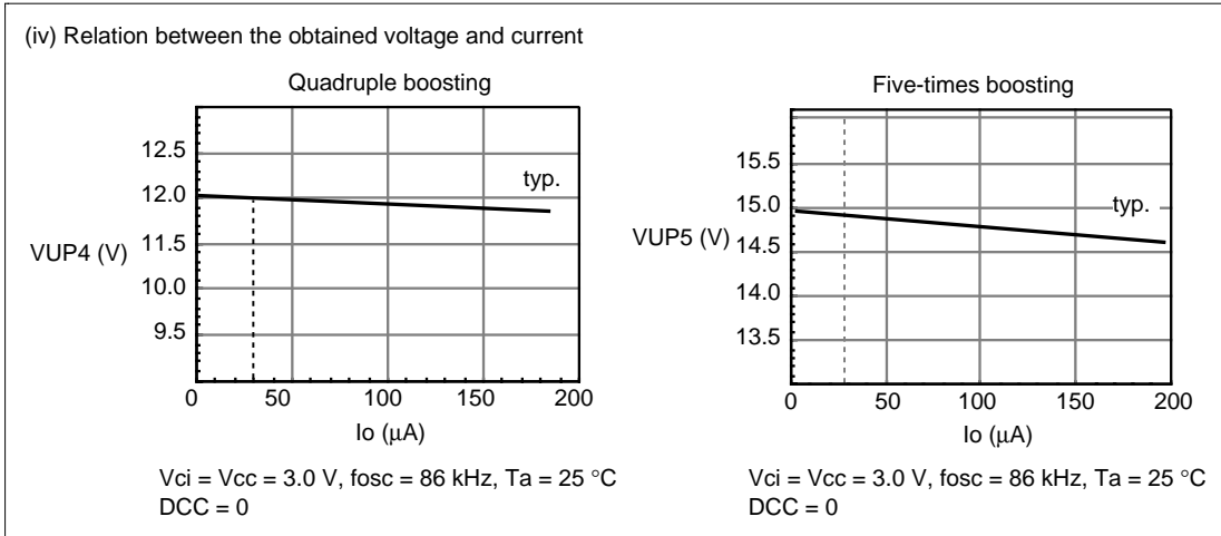
Figure 45 Booster (cont)
