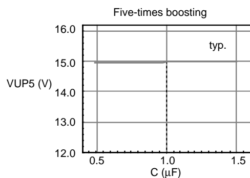
Figure 45 Booster (cont)
