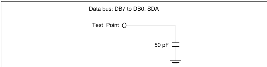
Figure 46 Load Circuit
