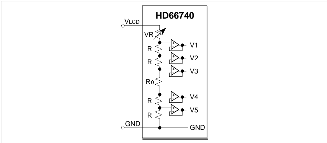
Figure 5 Contrast Adjuster
