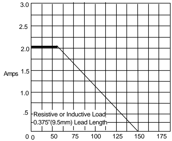
Average Forward Rectified Current - Amperes versus Ambient Temperature - °C
