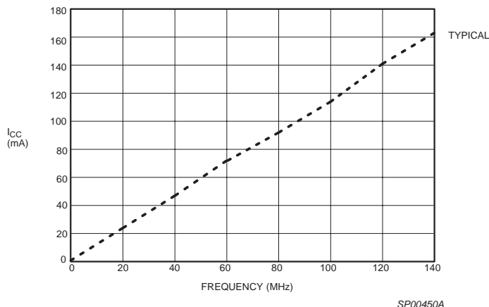
Figure 5: V CC vs. Frequency at V CC = 5.0V, 25°C
