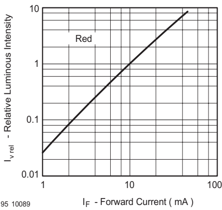
Figure 6. Relative Luminous Intensity vs. Forward Current
