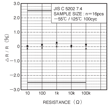
Fig.10 Temperature cycling
