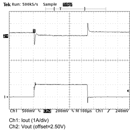
Load Transient
