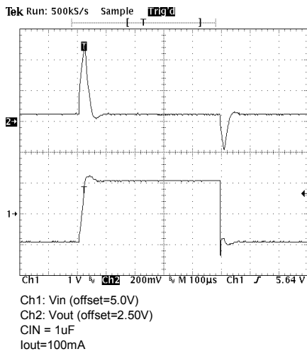
Line Transient
