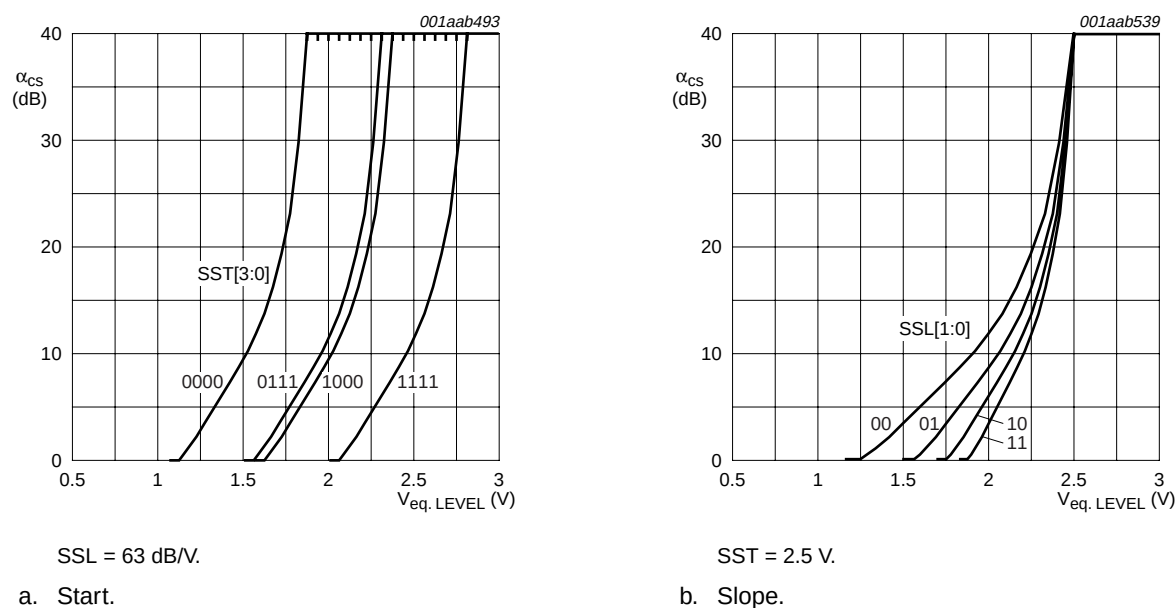
Fig 25. Stereo Noise Control (SNC) start and slope settings versus equivalent level voltage; SNC detector (level, USN and WAM), USN detector and WAM detector
