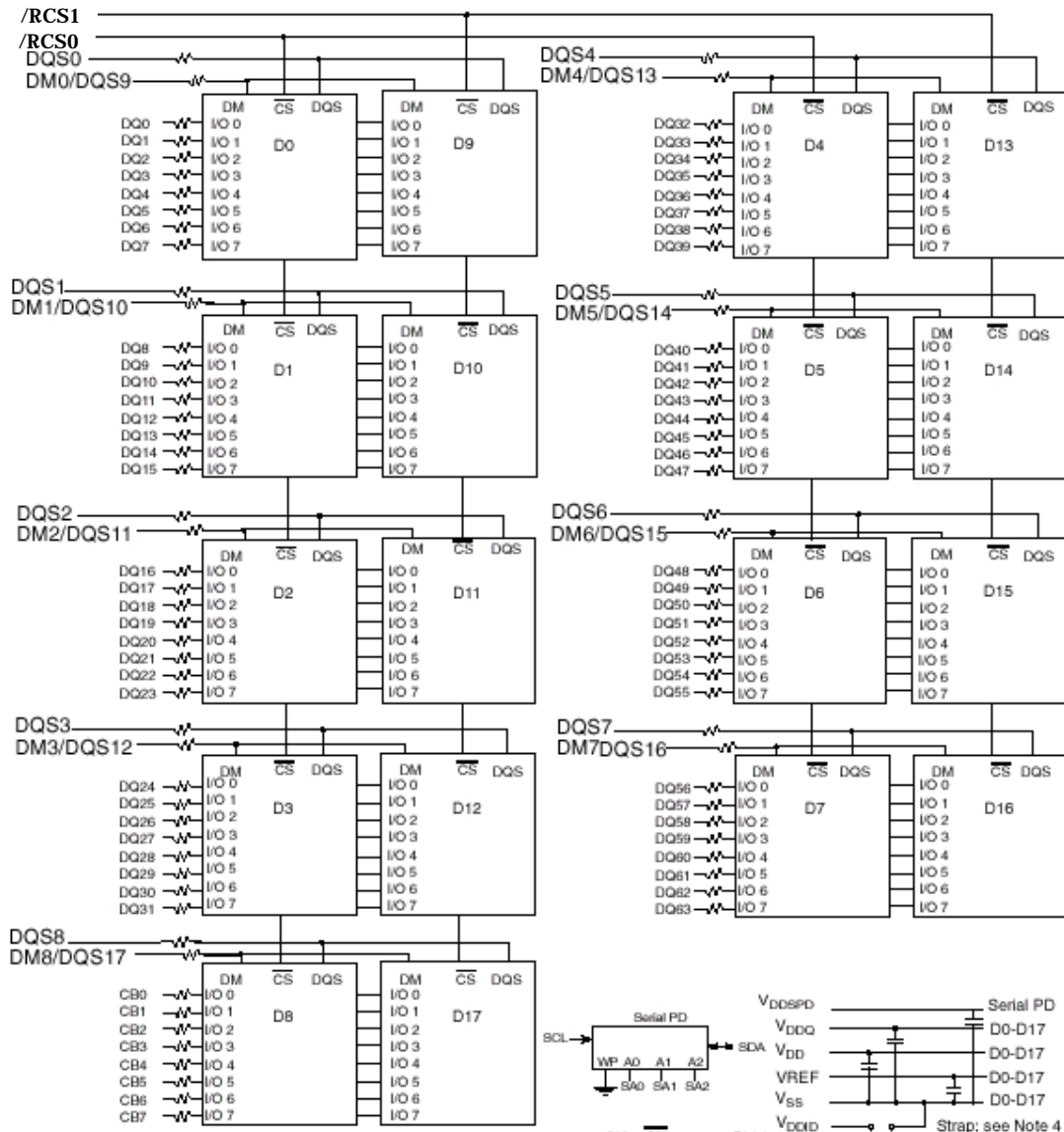
* Wire per Clock Loading Table/Wiring Diagrams
