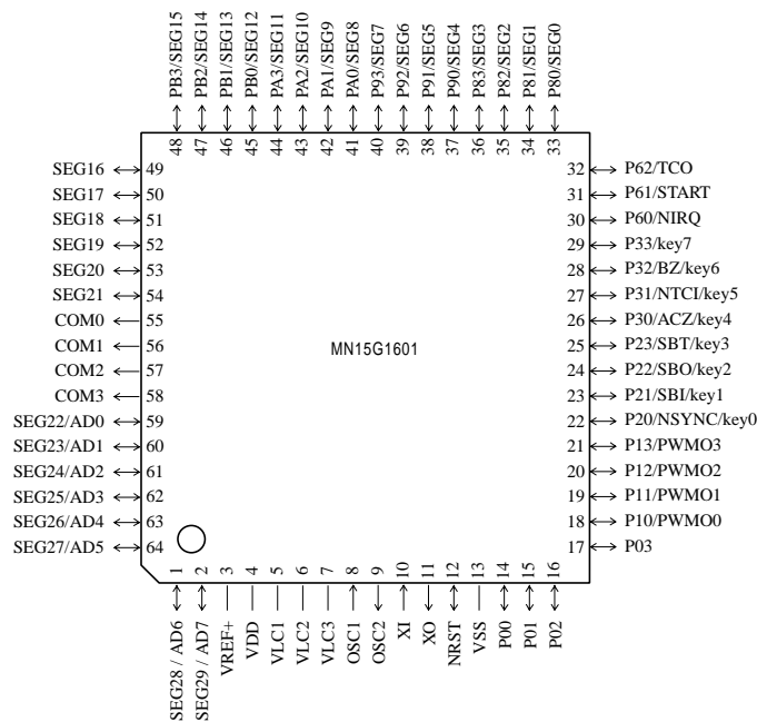
LQFP064-P-1414 *Lead-free
