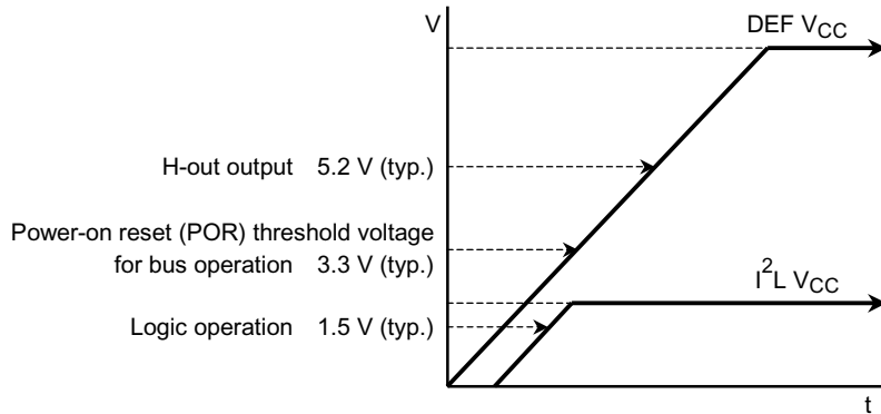
Figure 2 Timing from immediately after power-on to time at which H-out is output (at T_a = 25^\circ\text{C} )
