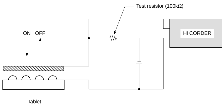
Measurement circuit
