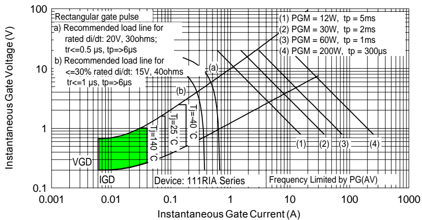
Fig. 9 - Gate Characteristics
